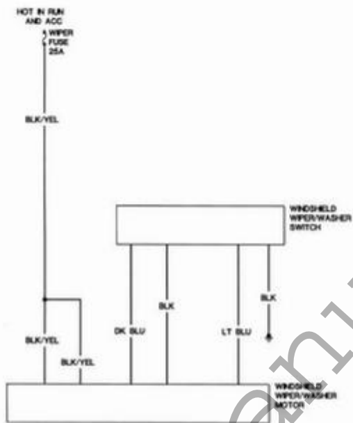
Body wiring diagram—1974-75 windshield wiper circuit
