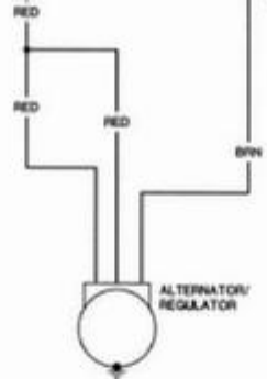
Body wiring diagram—1976 alternator/charging circuit
