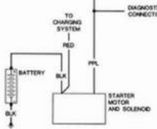
Body wiring diagram—1977-78 starter circuit
