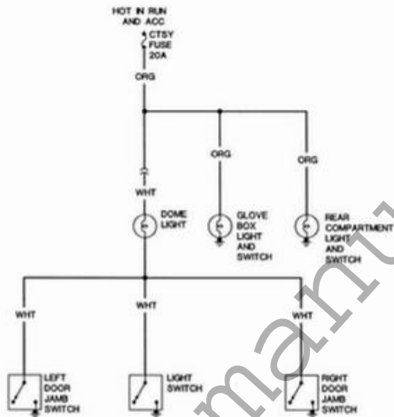
Body wiring diagram—1973 dome light circuit
