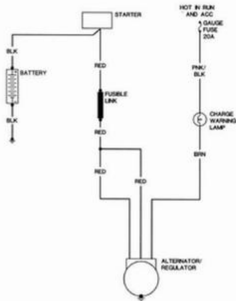
Body wiring diagram—1977-78 alternator/charging circuit
