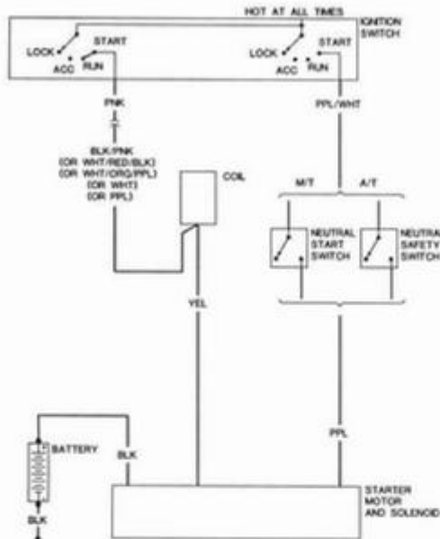
Body wiring diagram—1968-72 starter circuit
