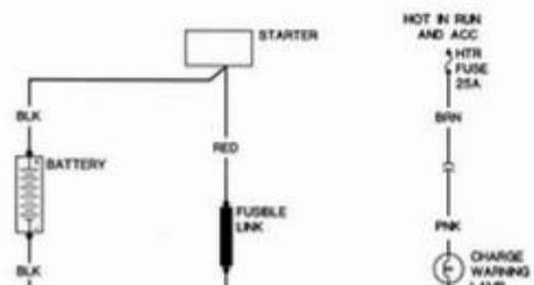
Body wiring diagram—1976 starter circuit
