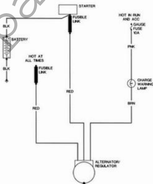
Body wiring diagram—1973 alternator/charging circuit
