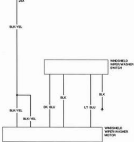
Body wiring diagram—1973 windshield wiper circuit
