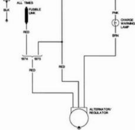
Body wiring diagram—1974-75 alternator/charging circuit
