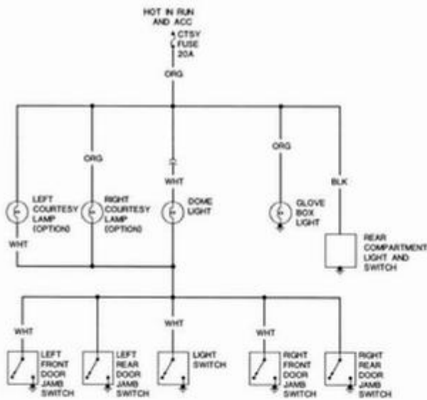
Body wiring diagram—1968-72 dome light circuit
