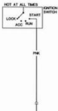
Body wiring diagram—1976 intermittent windshield wiper circuit
